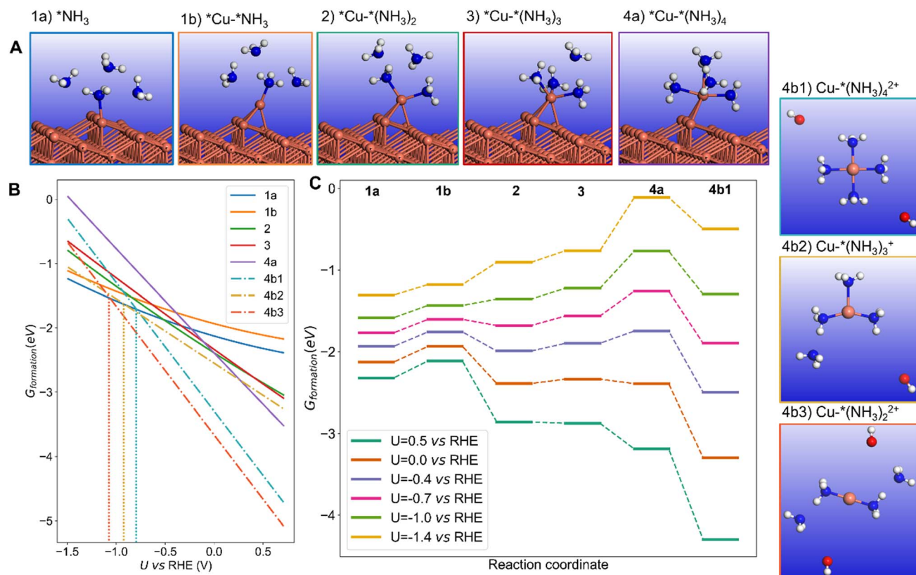
Fig. 4 Dissolution of the Cu(843) surface in the presence of NH 3 in water as a function of the potential, initiated at the kink site. (A) mechanisms and intermediates during the dissolution; 1a: adsorption of one NH 3 on the Cu kink site, 1b: diffusion of the NH 3 -capped kink site Cu atom forming a Cu adatom on the nearby terrace; adsorption of a second (2), third (3) and fourth (4a) NH 3 on the formed Cu adatom; (4b) Cu(NH 3 ) 4 2+ , Cu(NH 3 ) 3 + , and Cu(NH 3 ) 2 2+ complexes formation and detachment. (B) Free energy of the NH 3 induced surface or dissolved intermediates described in (A). The vertical blue dashed line describes the threshold potential above which the dissolved complex becomes most stable. (C) Potential dependent reaction pathway for NH 3 adsorption, surface complex formation and detachment, where labels refer to (A). pH equals 12.9.
